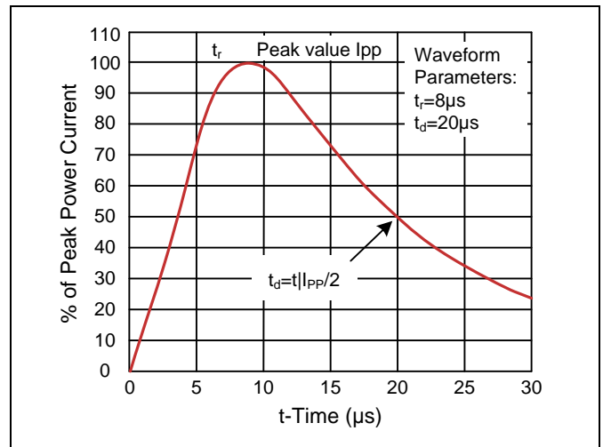
Figure 2. Pulse Waveforms
