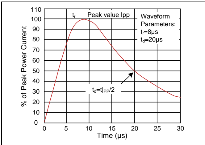
Figure 1. Pulse Waveform
